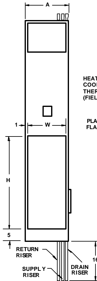
FRONT VIEW
