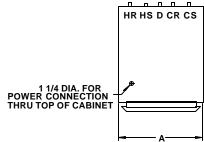
REAR RISER PORTS (ELEVATED VIEWS NOT SHOWN)
