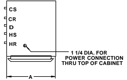
LEFT SIDE RISER PORTS (ELEVATED VIEWS SHOWN)
