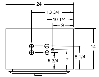
300, 400, 500, & 600 CFM UNITS
