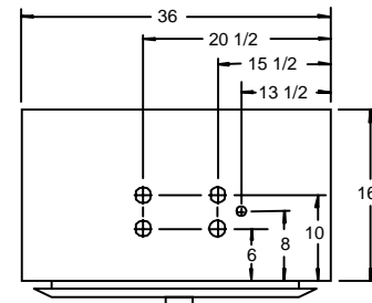
1200 & 1600 CFM UNITS
