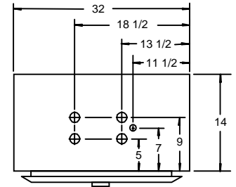
800 & 1000 CFM UNITS
