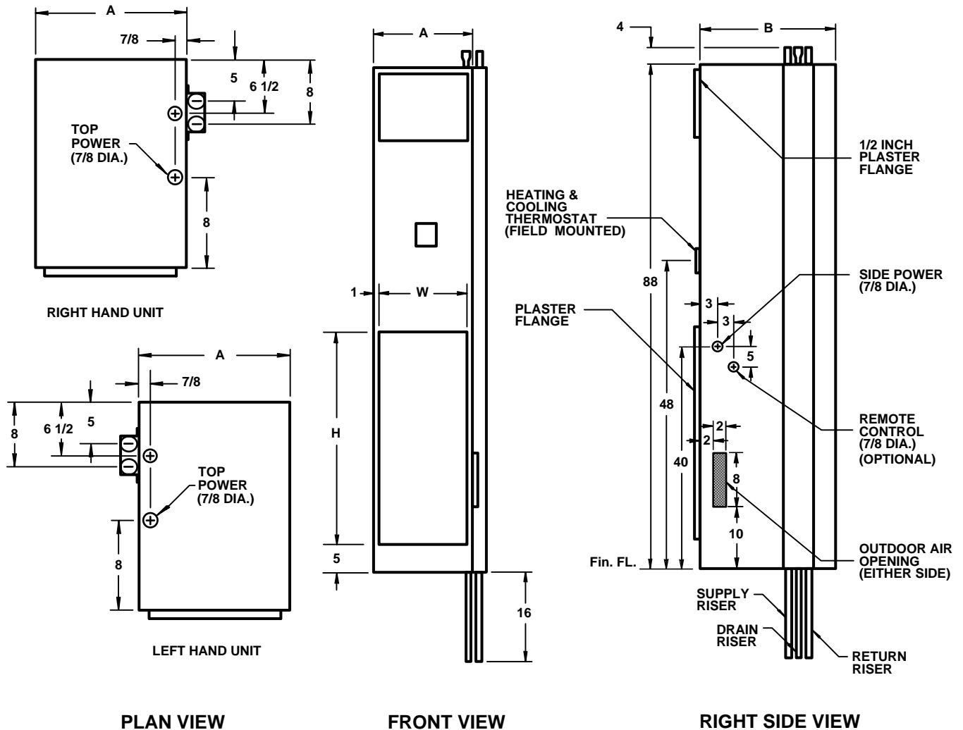
PLAN VIEW
