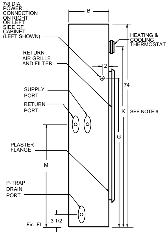
LEFT SIDE VIEW SIDE RISERS L.H. SHOWN
