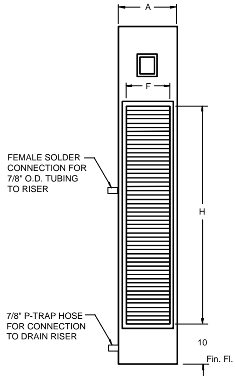
FRONT VIEW SIDE RISERS L.H. SHOWN
